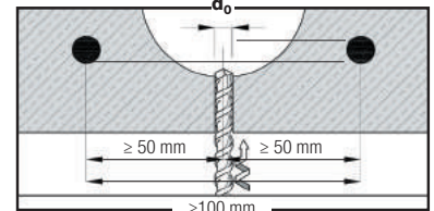
3. Make a cylindrical hole.
